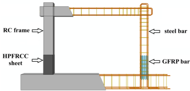
Fig. 1. Details of the numerical model of the strengthened RC frames at the column-base region.
