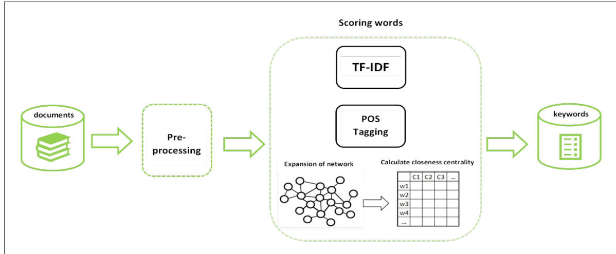
Fig. 1. Stages of Keyword Extraction
