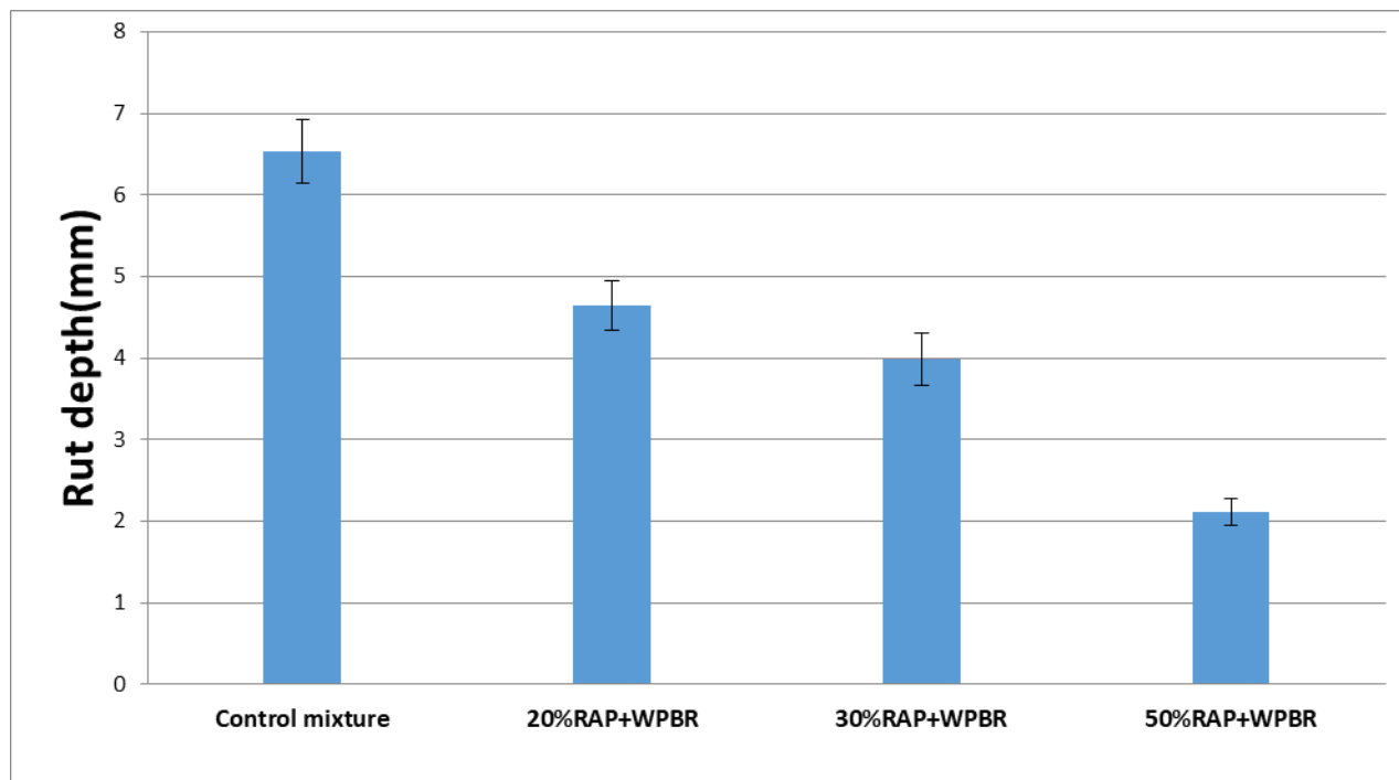
Fig. 3. Results of rut depth.
