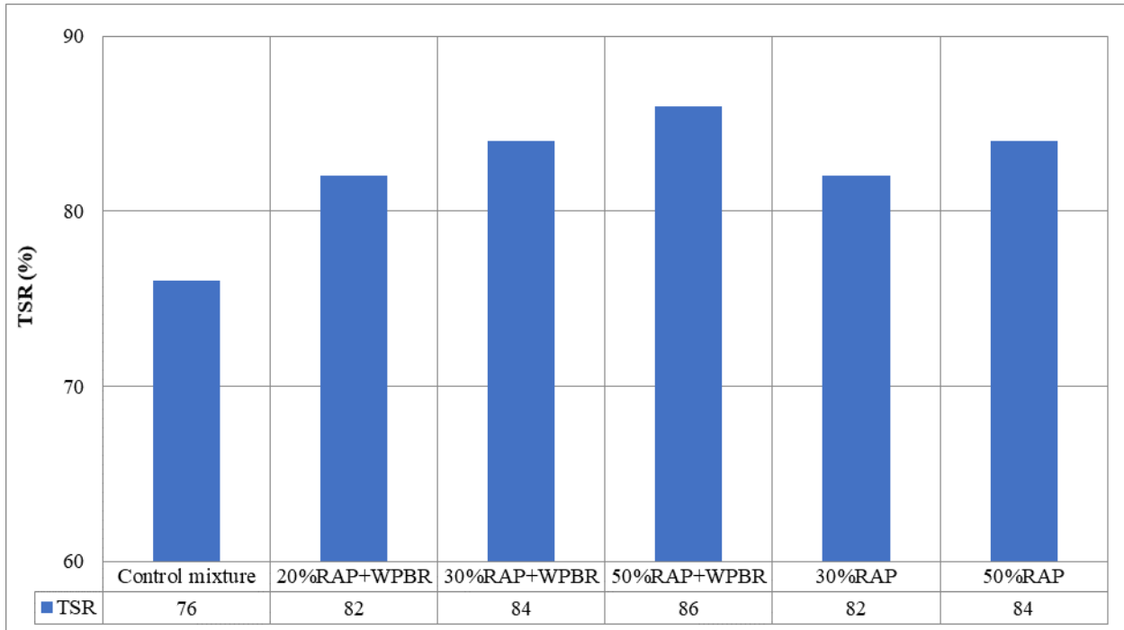
Fig. 2. TSR value of all mixtures.
