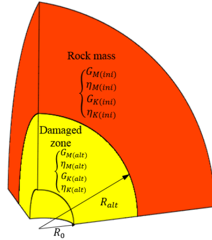
Figure 1. EDZ around the spherical cavity
