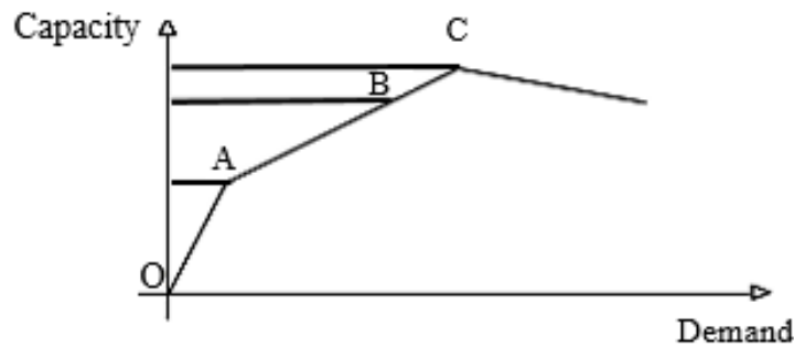
Fig. 1. Behavioral diagram of the reinforced concrete cross-section under loading
