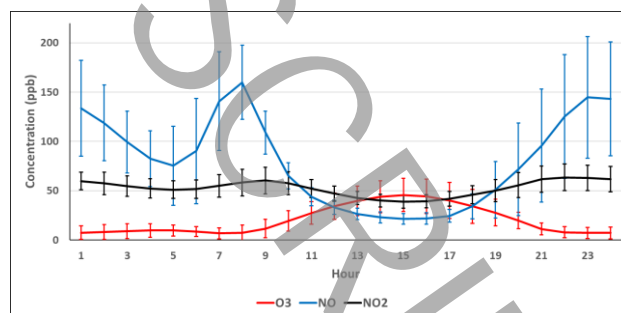
Figure1: cumulative average of NO, NO_2 , and O_3
