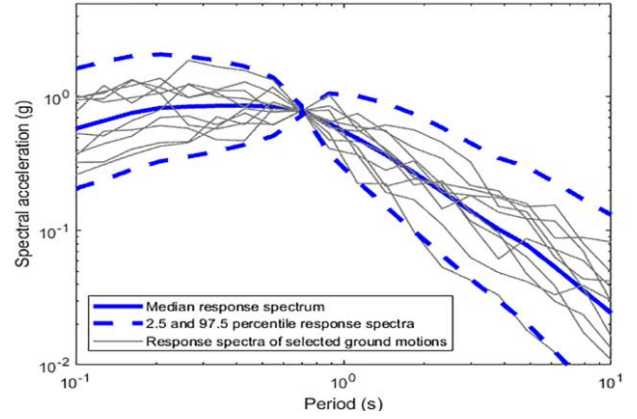
Figure 2. Response spectra of selected ground motions
