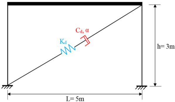
Figure 1. Studied shear frame
