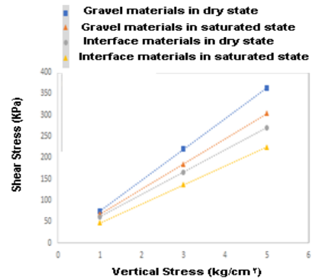
Figure 3. Changes in residual shear stress versus vertical stress at 60% relative density
