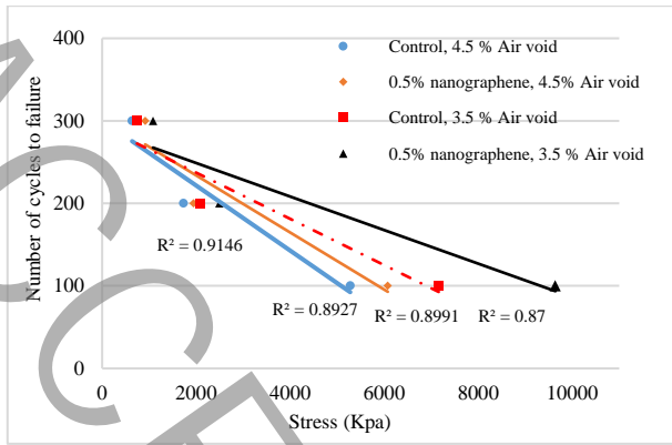
Figure 2 ITF test results
