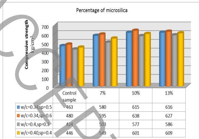
Figure 1: Effect of microsilica on compressive strength of 28 days of concrete
