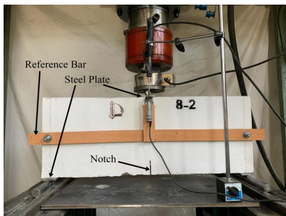
Figure 1. Details of Fracture Test
