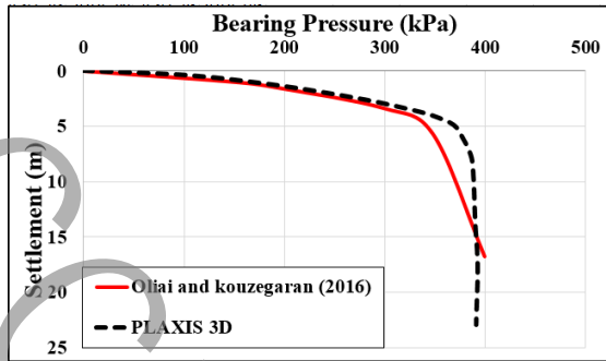
Figure 1. Comparison of the PLAXIS 3D results, obtained in this study, with the Oliaei and Kouzegaran (2016)
