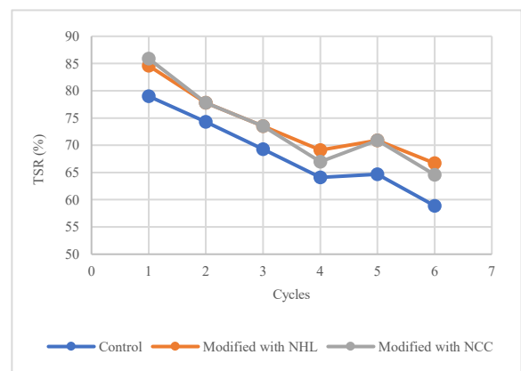
Fig. 2. Indirect Tensile Resistance Ratio (TSR) of AC 85-100
