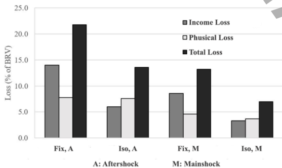
Figure 3. Effects of considering aftershocks in the final estimated seismic risk.
