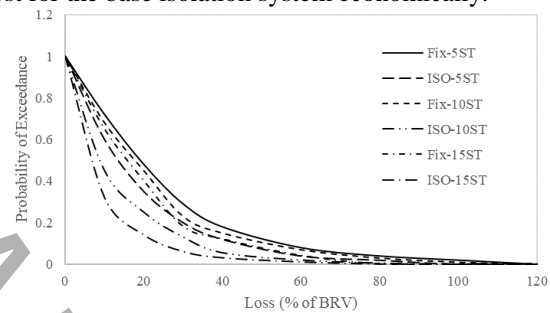
Figure 1. Exceedance probability curve of the estimated loss value of 5-, 10-, 15-story buildings with/without lead rubber bearing isolation system.
