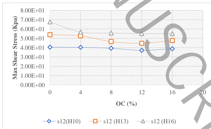
Figure 4. the changes of maximum shear stress against the changes of oil contamination in the heights of 10, 13, and 16m
