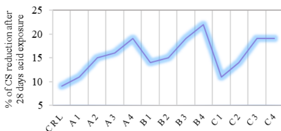
Figure 4- the percentage of CS reduction after 28 days at sulfuric acid exposure
