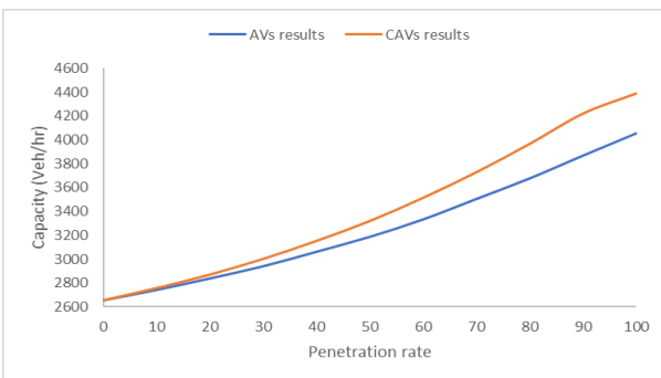
Figure 3. Impact of AVs on capacity of merge section
