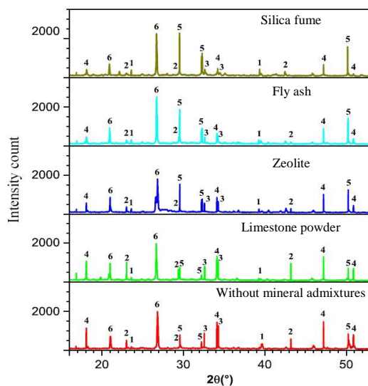
Figure 3. XRD spectra for the prepared 28-day concrete specimens with and without mineral admixtures (replacement level is 5%, 1: C_3AH_6 , 2: CaCO_3 , 3: C_2S/C_3S , 4: Ca(OH)_2 , 5: C-S-H, 6: SiO_2 )
