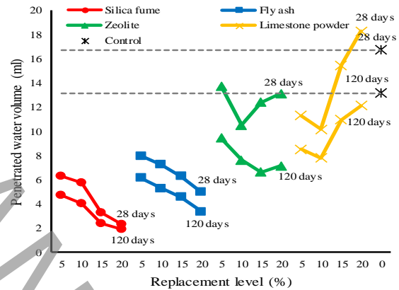
(a) Penetrated water volume measured for the prepared concrete specimens
