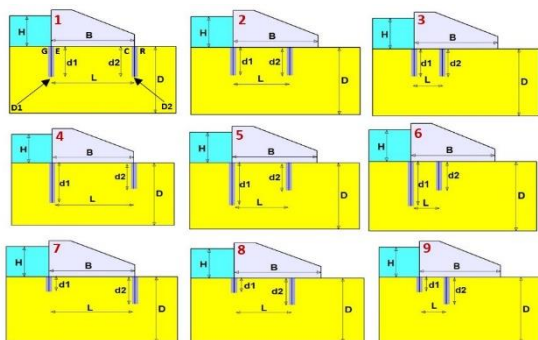
Figure 1 Illustrations of different configurations of double cutoff walls under the hydraulic structure
