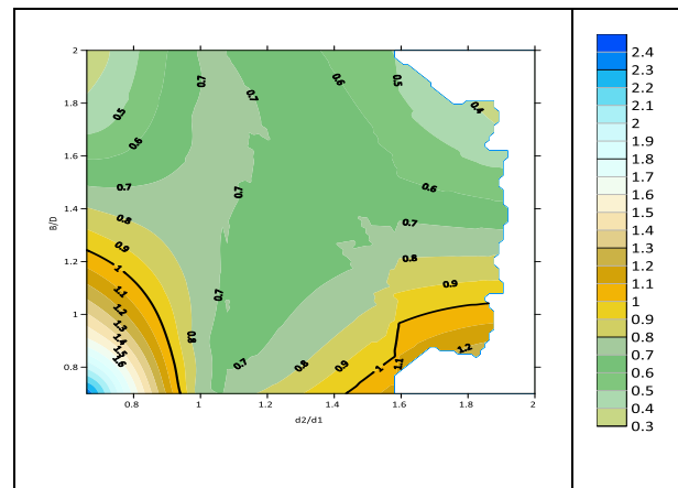
Figure 2 Contours of U/U_0 as a function of d_2/d_1 and B/D
