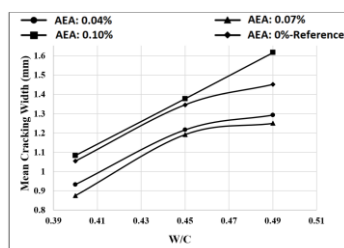
Figure 2. Change of mean cracking width of air-entrained concrete pavement mixtures relative to W/C
