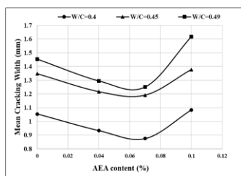
Figure 1. Change of mean cracking width of air-entrained concrete pavement mixtures relative to air-entraining agent content
