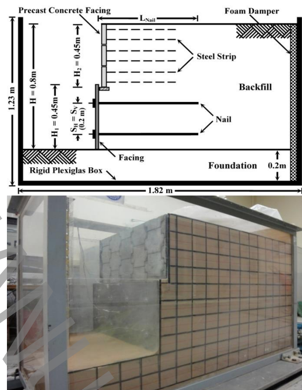
Figure 1. The schematic geometry and pictures of hybrid wall model
