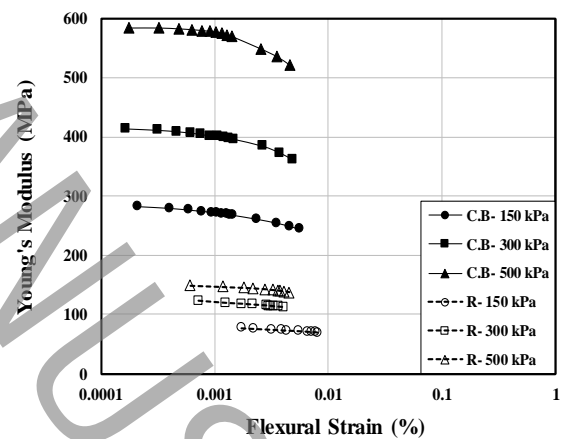
Figure 1: Effects of Reconstitution and confining pressure on Young's Modulus
