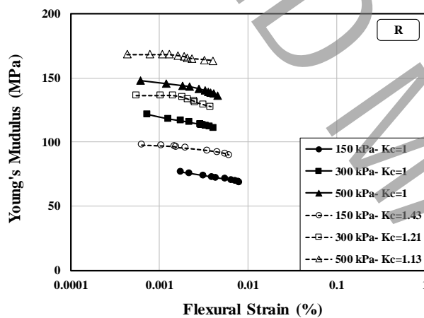
Figure 3: Effect of stress anisotropy on Young's modulus in reconstituted sample
