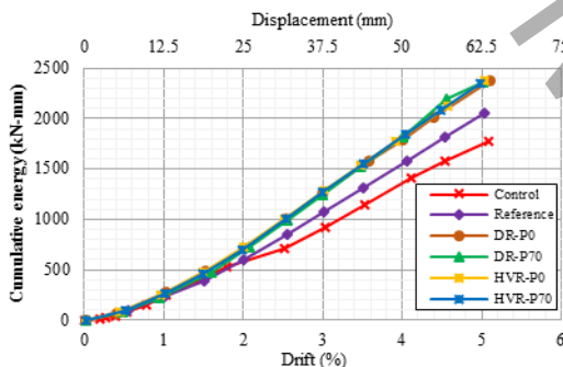
Figure 4. Comparison of cumulative energy dissipation up to 5% drift
