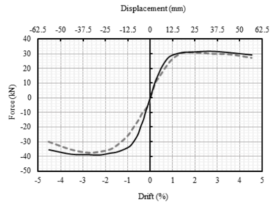
Figure 1. Comparison of experimental [8] and analytical envelope curve
