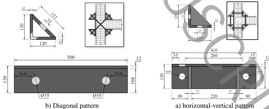
Figure 2. Detail of retrofitting patterns (all dimensions are in mm)
