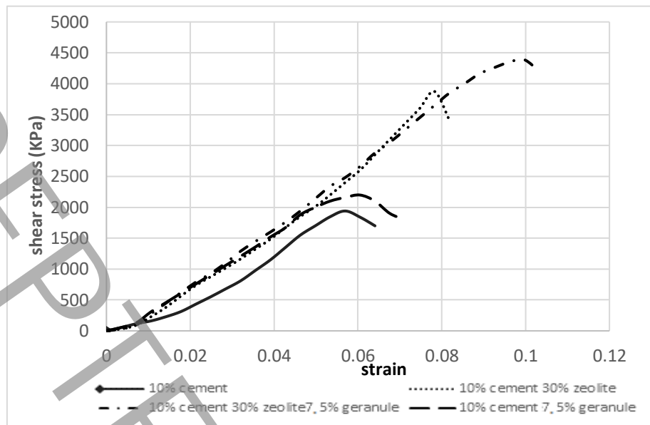
Figure 1: Effect of zeolite and granule on stress-strain behavior.
