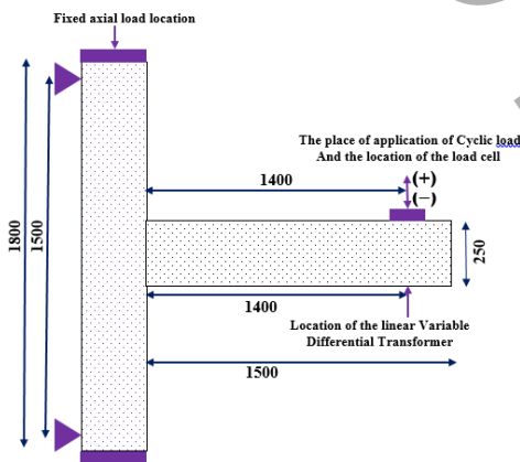
Figure 2. Schematic view of the test configuration (all dimensions are in millimeters)
