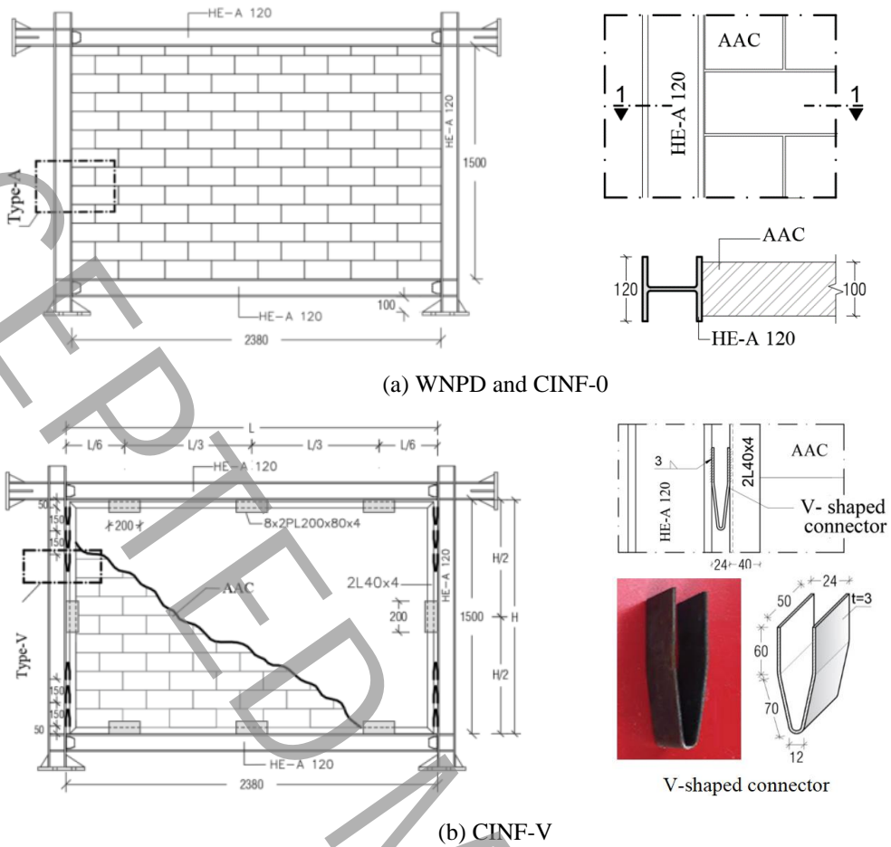
Figure 1. Detailed dimensions and configurations of specimens (unit: mm)
