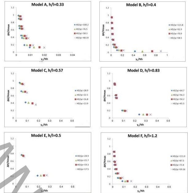
Figure 2. Variation of \frac{\Delta H}{H_{max}} in terms of \frac{y_c}{Nh} for different models of the present study
