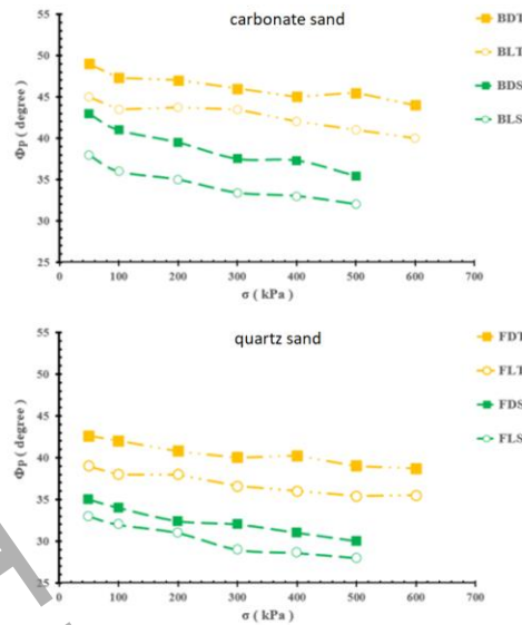
Figure1. Internal friction angle versus confining stress
