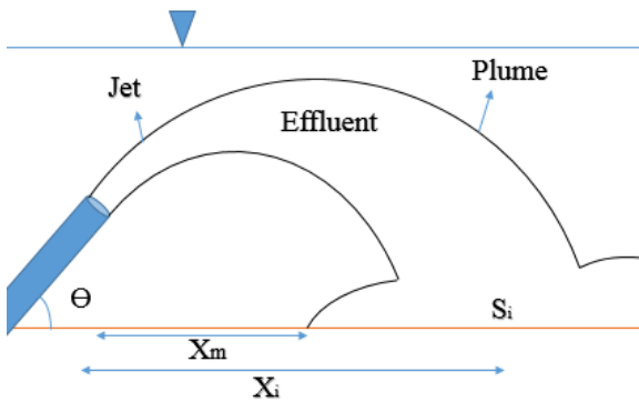
Figure 1. Schematic of submerged discharge of dense effluent. X_m is the horizontal location of the centerline peak, X_i is the horizontal location of the impact point, S_i is the minimum centerline dilution at the impact point, and \theta is the discharge angle relative to the horizon.
