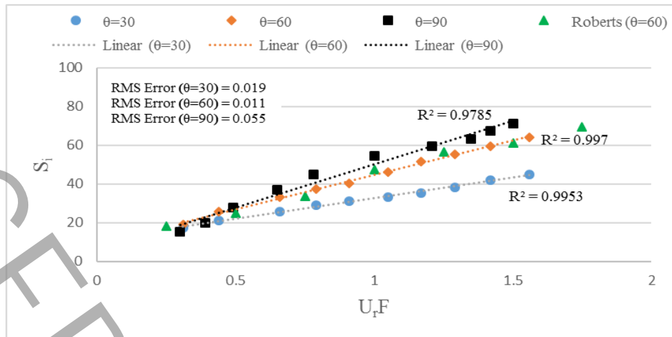
Figure 2. Comparison of dilution of dense effluent with different discharge angles in the case of \phi = 0 (co-flow).
