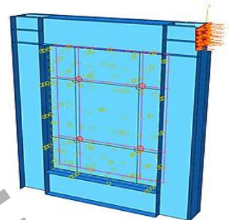
Fig 1: Boundary conditions of model floor trapping and loading method
