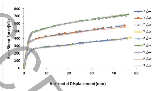
Fig 2: Base cut-displacement diagram of 9 models of the first group ( b / d = 0.75 )
