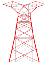
18) The optimal 47-member truss
