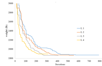
Figure 17) Diagram of the convergence history of the 47-member structure
