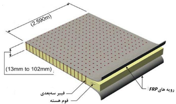
Figure 1: Schematic of 3D FRP sandwich panel [11]
