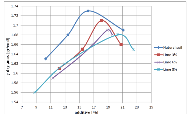
Figure 4- maximum dry density versus optimal moisture content for different percentages of lime
