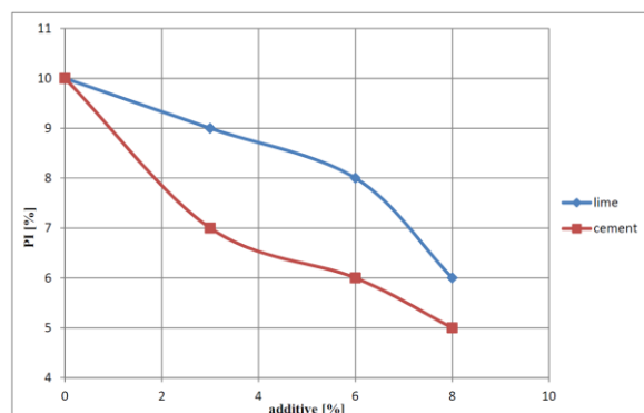
Figure 1- plasticity index diagram for soil mixed with different percentages of lime and cement
