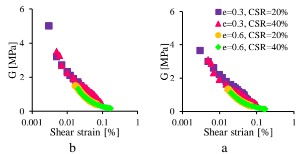
Figure 1. Variation of shear modulus with shear strain for spherical (a) and non-spherical (b) particles specimens
