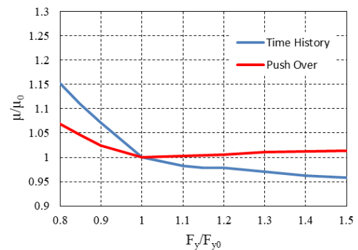
Figure 1: Average ductility demand values for different strength values under the nonlinear dynamic and static analysis.
