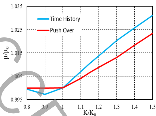
Figure 2: Average ductility demand values for different stiffness values under the nonlinear dynamic and static analysis.
