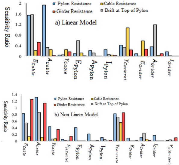
Figure 3. Sensitivity ratios of girder, cable, pylon to input parameters
