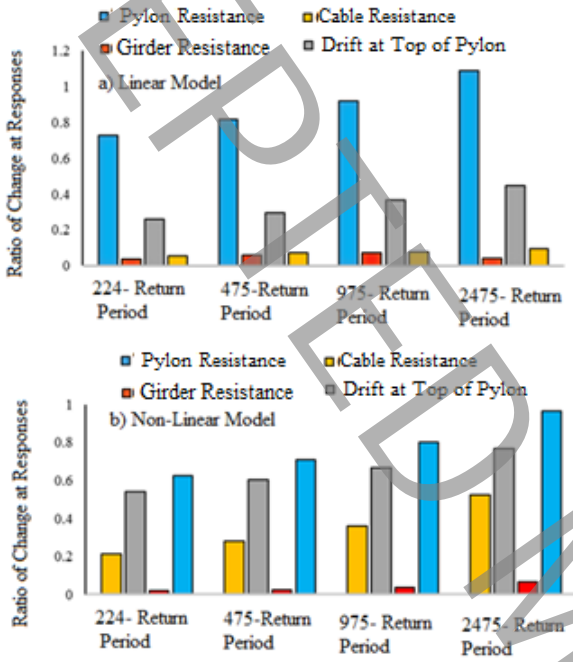
Figure 2. The ratio of change at responses for various seismic levels
