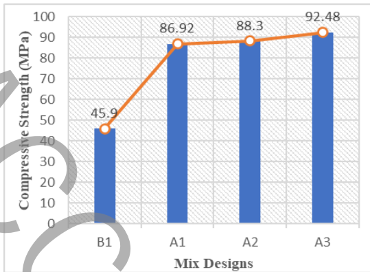
Figure 1. Comparative diagram of compressive strengths
