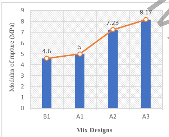
Figure 3. Comparative diagram of modulus of ruptures
