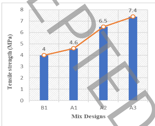
Figure 2. Comparative diagram of tensile strengths
