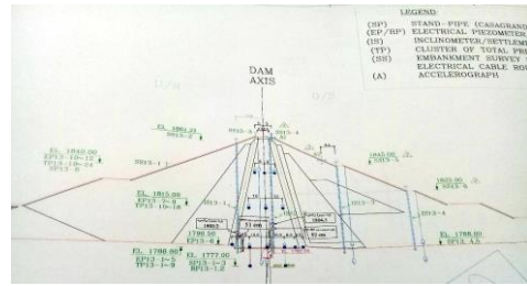
Figure 1. Typical cross-section of Kamal-Saleh rockfill dam [8]
