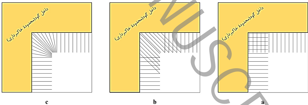
Figure 3. Various modes for soil nails azimuth in the affected zone: a) No azimuth b) Constant azimuth c) Variable azimuth
