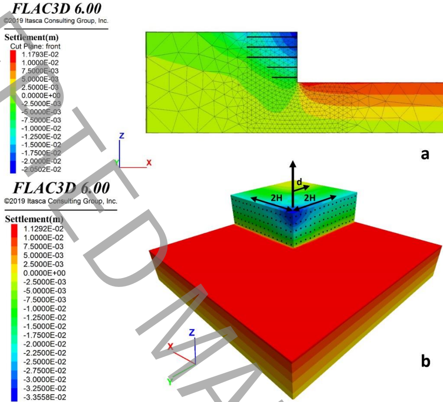
Figure 1. The 2D (a) and 3D (b) contours of settlement for the 10m soil-nailed wall with the weak soil
