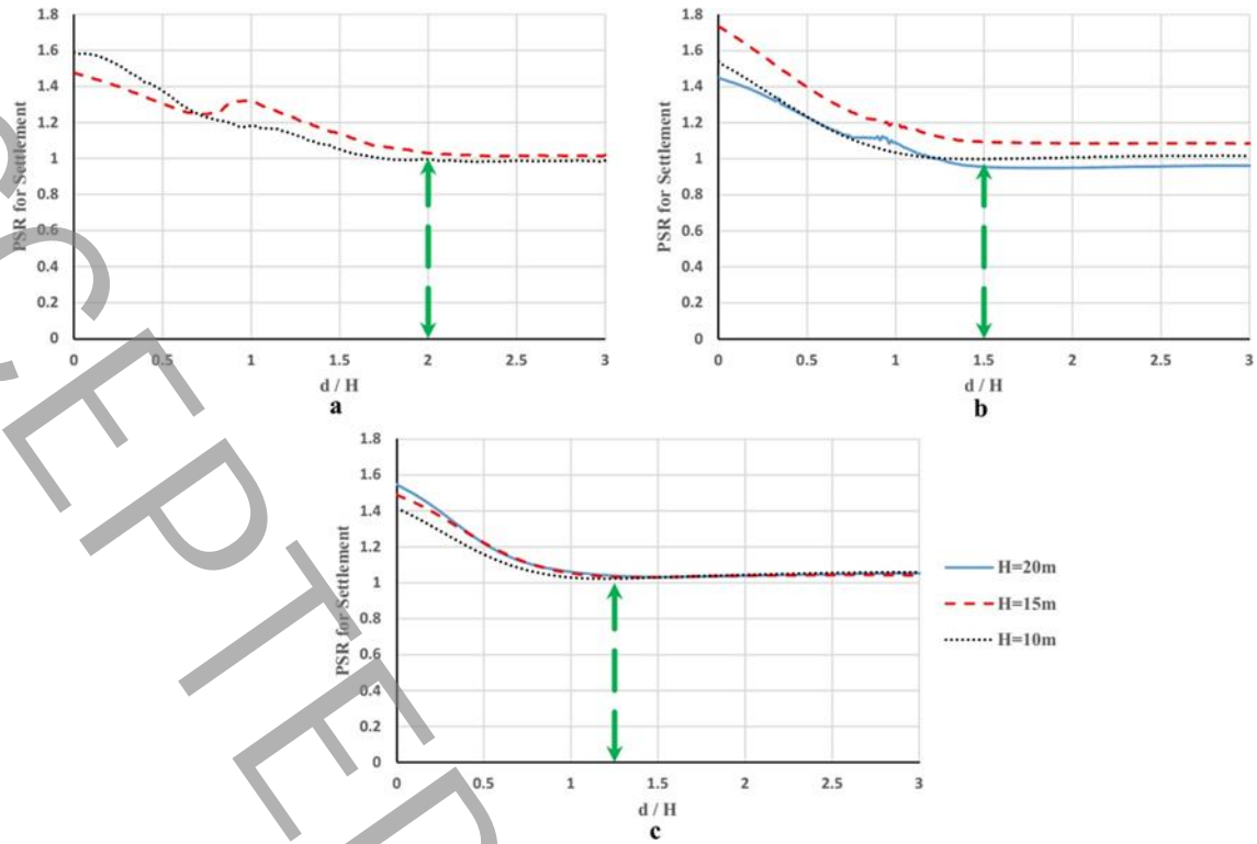
Figure 2. Variations of PSR values versus d/H for the models: a) Weak soil b) Medium soil c) Strong soil
