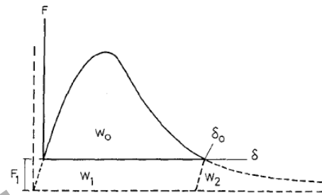
Figure 1. Force - displacement curve used to calculate the fracture energy of samples
