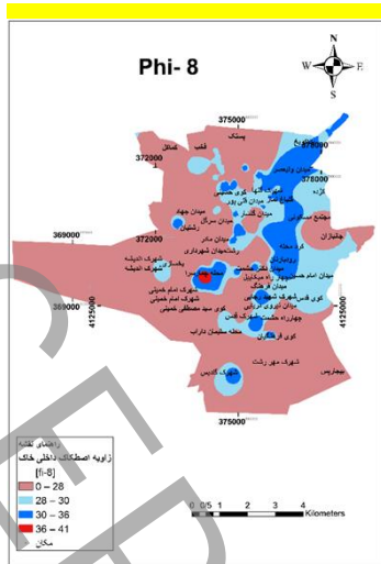
Figure 3. Rasht internal friction angle zoning map at a depth of 8 m
