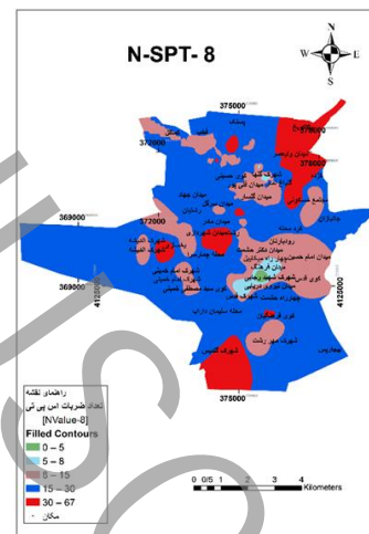
Figure 2. Rasht SPT zoning map at a depth of 8 m
