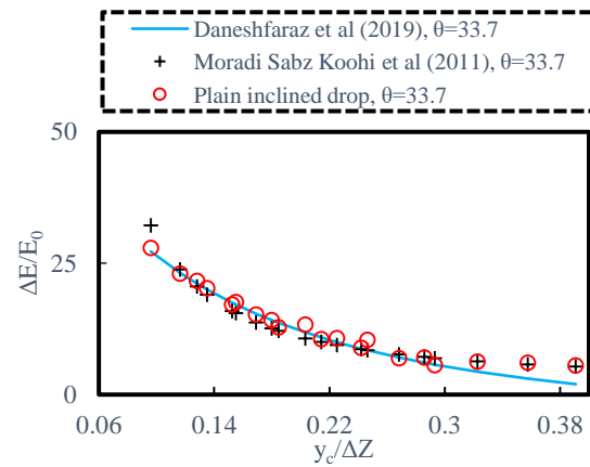
Figure 1. compares the relative energy dissipation changes of the research studies [1] and [2]
