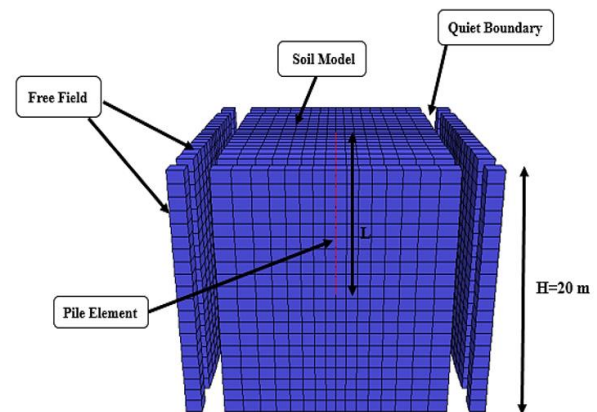
Figure 2. Schematic view of created model
