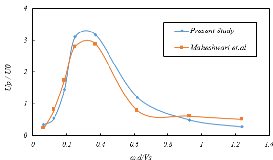
Figure 1. Response of pile head in dynamic loading
