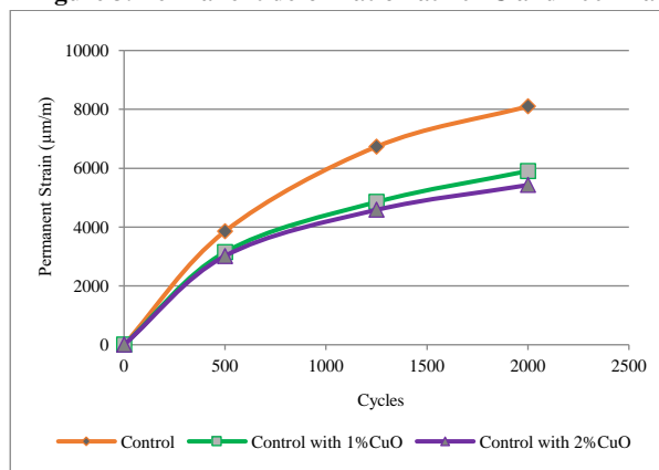
Figure 4. Permanent deformation at 40 °C and 400 kPa
