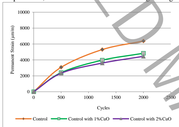
Figure 3. Permanent deformation at 40 °C and 200 kPa
