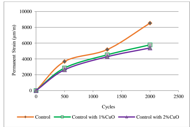
Figure 5. Permanent deformation at 60 °C and 200 kPa
