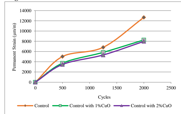
Figure 6. Permanent deformation at 60 °C and 400 kPa
