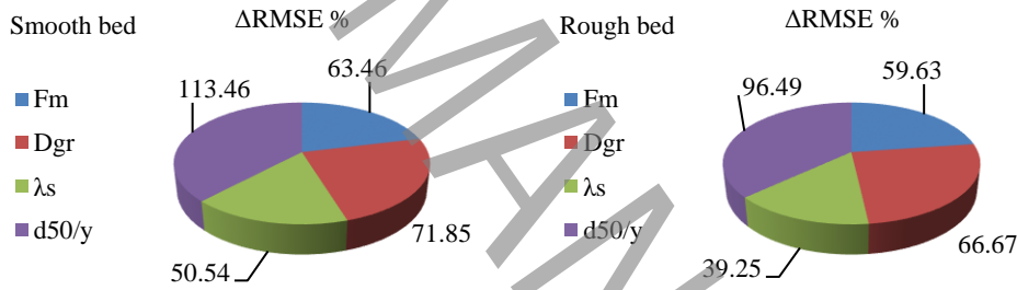
Figure 2. Relative significance of each of input parameters of the best model
