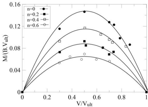
Fig. 3. Failure envelopes of the ring footing in M/BV_{ult} - V/V_{ult}
