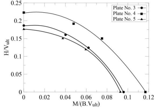
Fig. 4. Failure envelopes of the ring footing in H/V_{ult} - M/BV_{ult}
