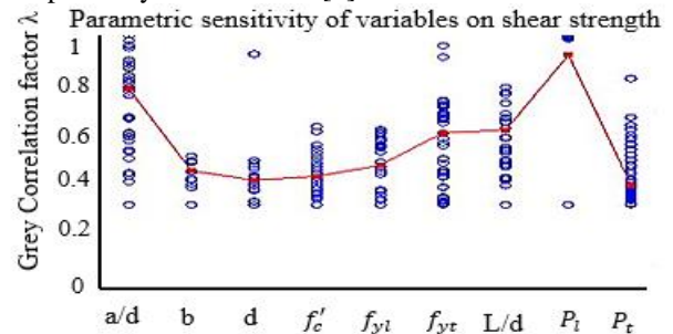
Figure 1. Parametric sensitivity analysis for key variables of shear capacity
