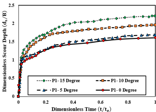
Figure 1. Time development scour of the first type of pier under zero, 5, 10 and 15-degree angles with the flow direction
