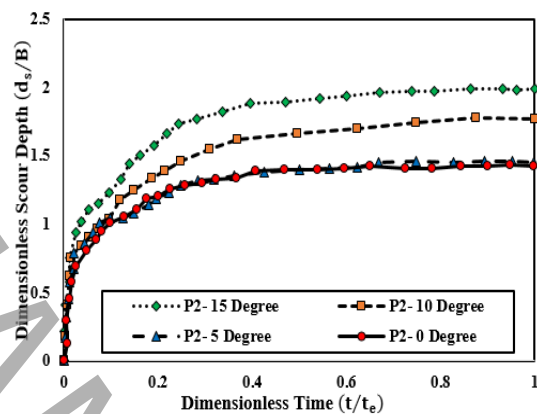
Figure 2. Time development of scour the second type of pier under zero, 5, 10 and 15-degree angles with the flow direction
