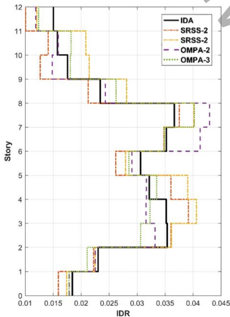
Figure 2. Inter-story drift profiles of 12 story model
