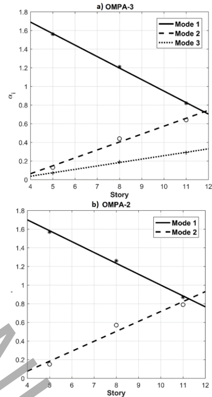
Figure 2- The resulted \alpha_i coefficient values in terms of Story number: a) OMPA by 3 modes, b) OMPA by 2 modes.
