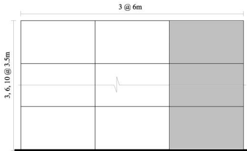
Figure 1. The schematic elevation of the studied frames
